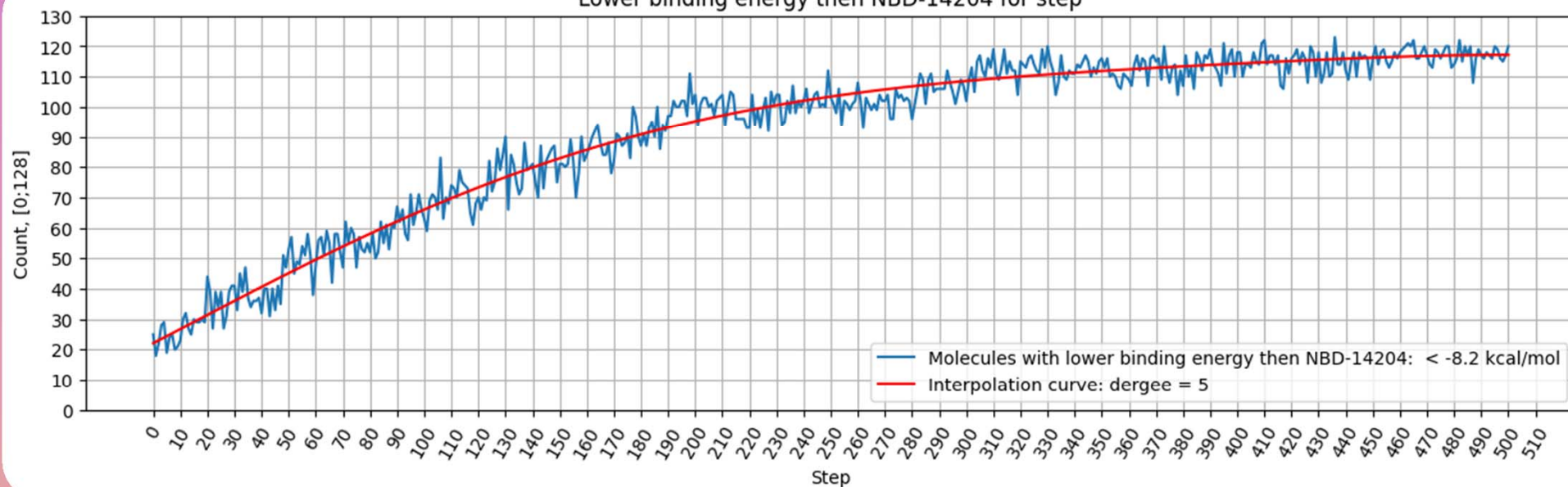
Lower binding energy then NBD-14204 for step
